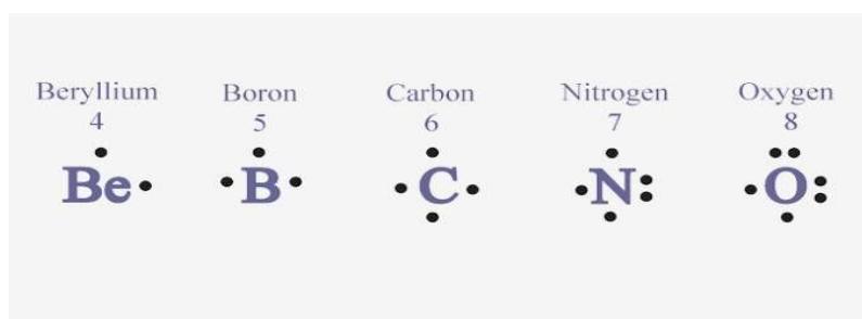
Lewis structures of elements with atomic number 5-8
